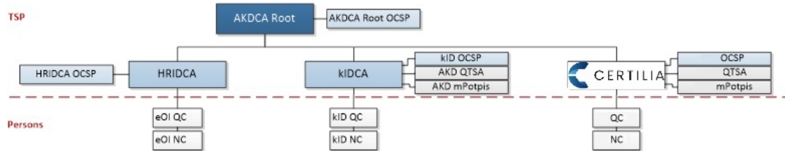
Figure 1: Hierarchical model AKD PKI
