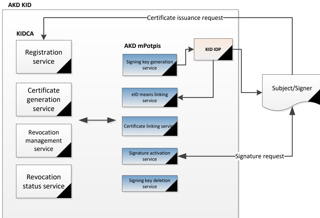
Figure 1a: AKD mPotpis (SSASC)
